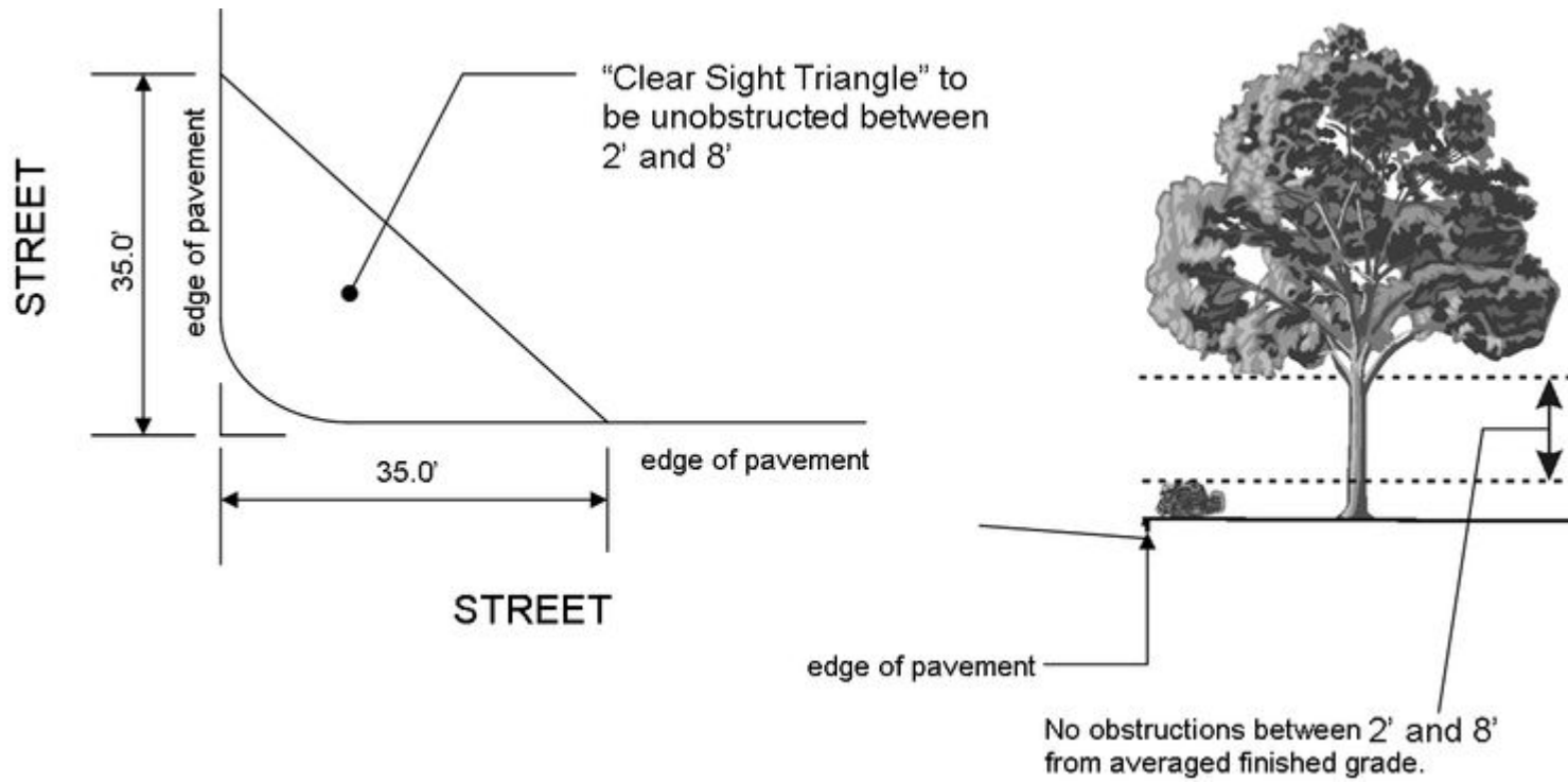
Picture 1. Visibility or Clear Sight Triangle
